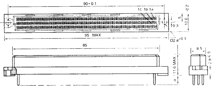
CONTACT ARRANGEMENT VIEW FROM TERMINATION SIDE
