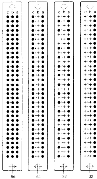
CONTACT ARRANGEMENT VIEW FROM TERMINATION SIDE
