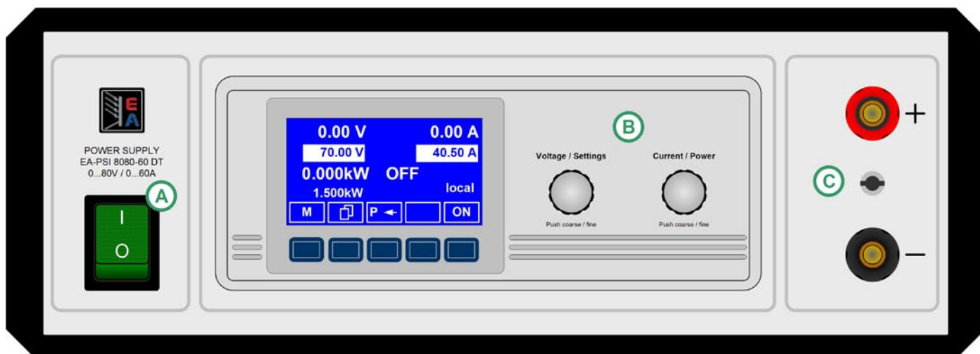
Figure 1. Front view
