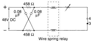
14. Pulse dialing test Tested sample: TX2-5V, 6 pcs (35 mA 48V DC wire spring relay load) Circuit
