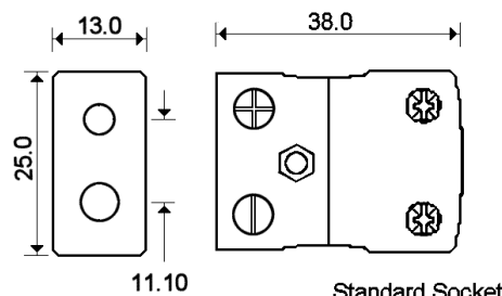
Standard Socket
