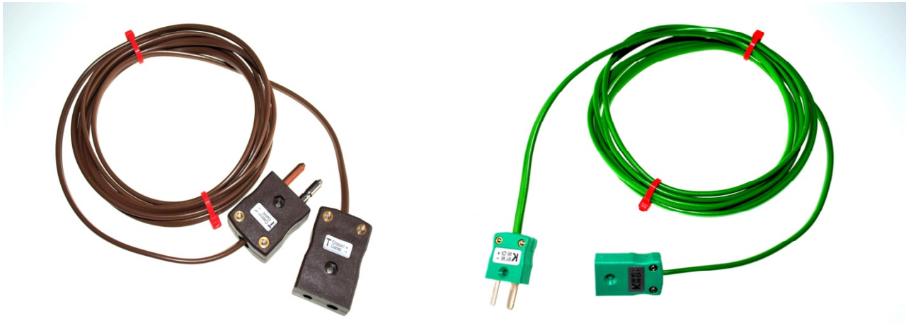
(Note: Illustration shows Type 'T' with standard connectors and Type 'K' with miniature connectors – for indication only)
