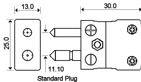
Standard Plug
