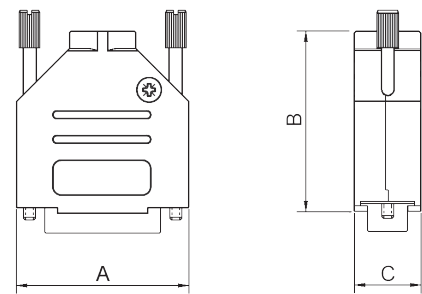
D-Sub-Hood
