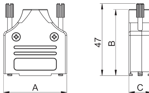
D-Sub-Hood
