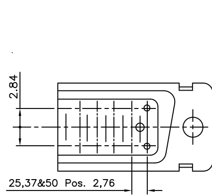
LAY OUT OF 50P CONNECTOR
