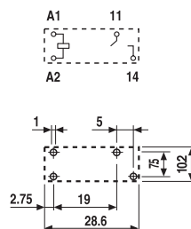
Copper side view
