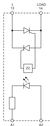
Simplified circuit diagram
