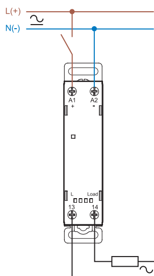
Single-phase connection (77.31...805x)
