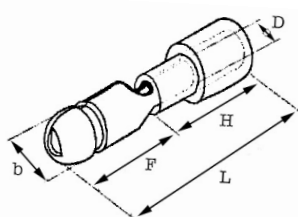
Round-Plug Bullet Connector Male
