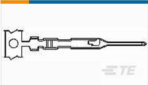
TE Part #1-104505-1 MTE PIN LP
