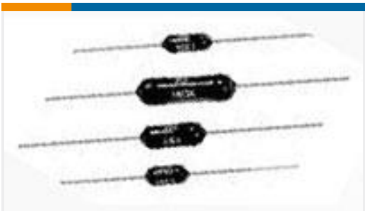
TE Part #8-1879621-3 H4P 27K 1% 50PPM
