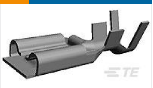
TE Part #175034-1 PL 187 REC 20-14 AWG 0.30 X 14.0 SS
