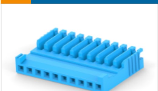
TE Part #1-281786-0 HE13/HE14 IDC Receptacle, SRST, AWG24-2
