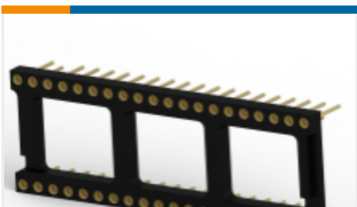
TE Part #1437538-3 DIP Socket: Standard, Screw Machine, Open, Gold
