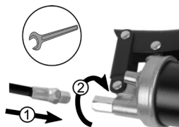
Figure 2 : Raccorder le tuyau
