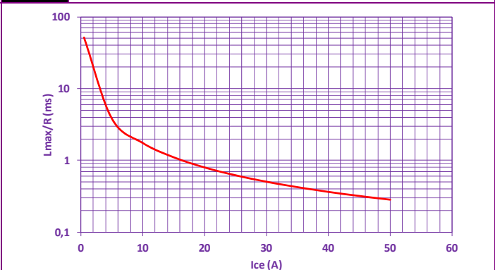
Fig. 10 MAXIMUM TIME CONSTANT WITH RL INDUCTIVE LOAD
