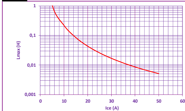
Fig. 9 MAXIMUM TOTAL INDUCTANCE (LOAD+LINE) ADMISSIBLE BY THE IGBT
