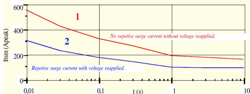
Fig.3 Surge current : I_{tsm} (A_{peak}) = f(t) for 50A models with I_{tsm} = 550\text{A}
