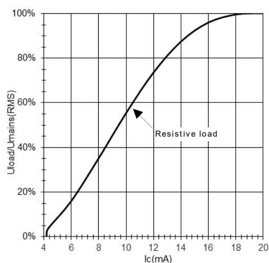
Fig.1 Transfer characteristic :
