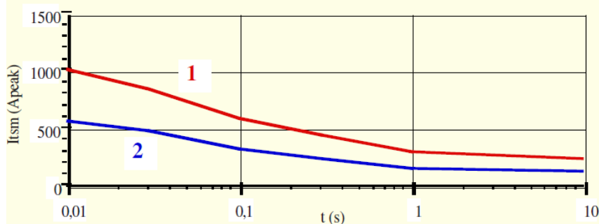
Fig.3 Surchage de courant : I_{tsm} (\text{Apeak}) = f(t)
