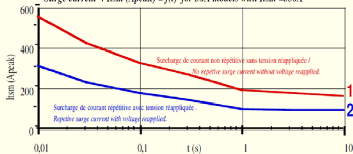
Fig.3 Surcharge de courant : I_{tsm} (A_{peak}) = f(t) pour modèle 50A ( I_{tsm} = 550A ) Surge current : I_{tsm} (A_{peak}) = f(t) for 50A models with I_{tsm} \approx 550A
