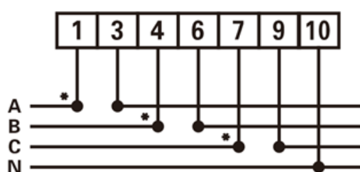
Figure 9 Three phase four wire: direct connect
