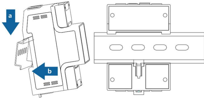
Figure 11 Installation Diagram
