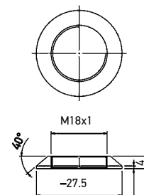
M18 FLARED PLASTIC NUT
