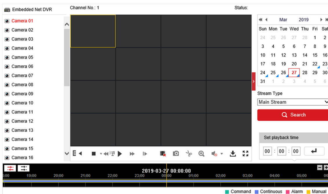
Figure 9-3 Playback
