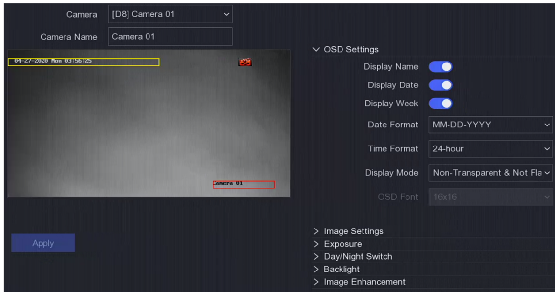
Figure 6-11 OSD
