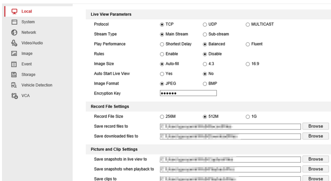
Figure 9-4 Configuration
