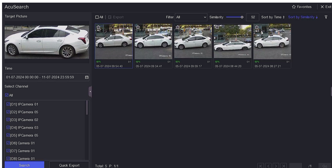
Figure 3-5 AcuSearch
