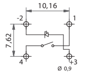
Single LED
