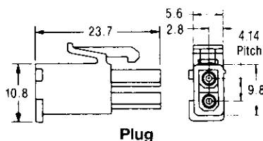
Plug
