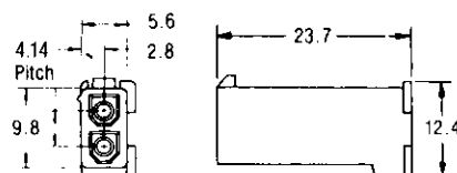
Cap (Free-Hanging)
