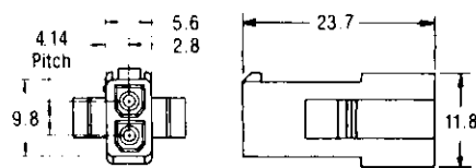
Cap (Panel Mount)
