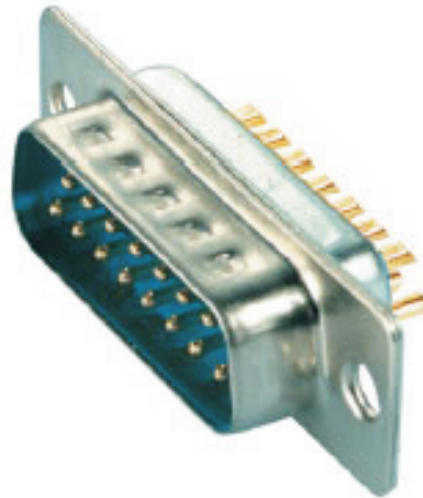
Sub – D 15 PIN plug with solder clips, gold plated
