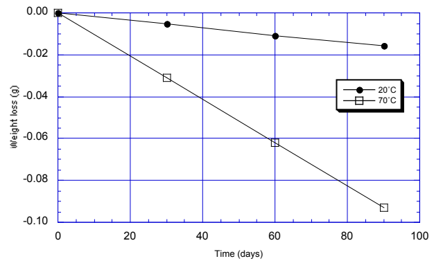
Figure 22 - Water loss test
