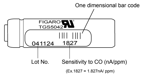
Figure 23 - TGS5042 markings (NOTE: UL Mark may appear on shrink tube)
