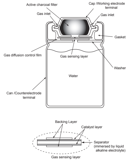
Figure 1 - Sensor structure
