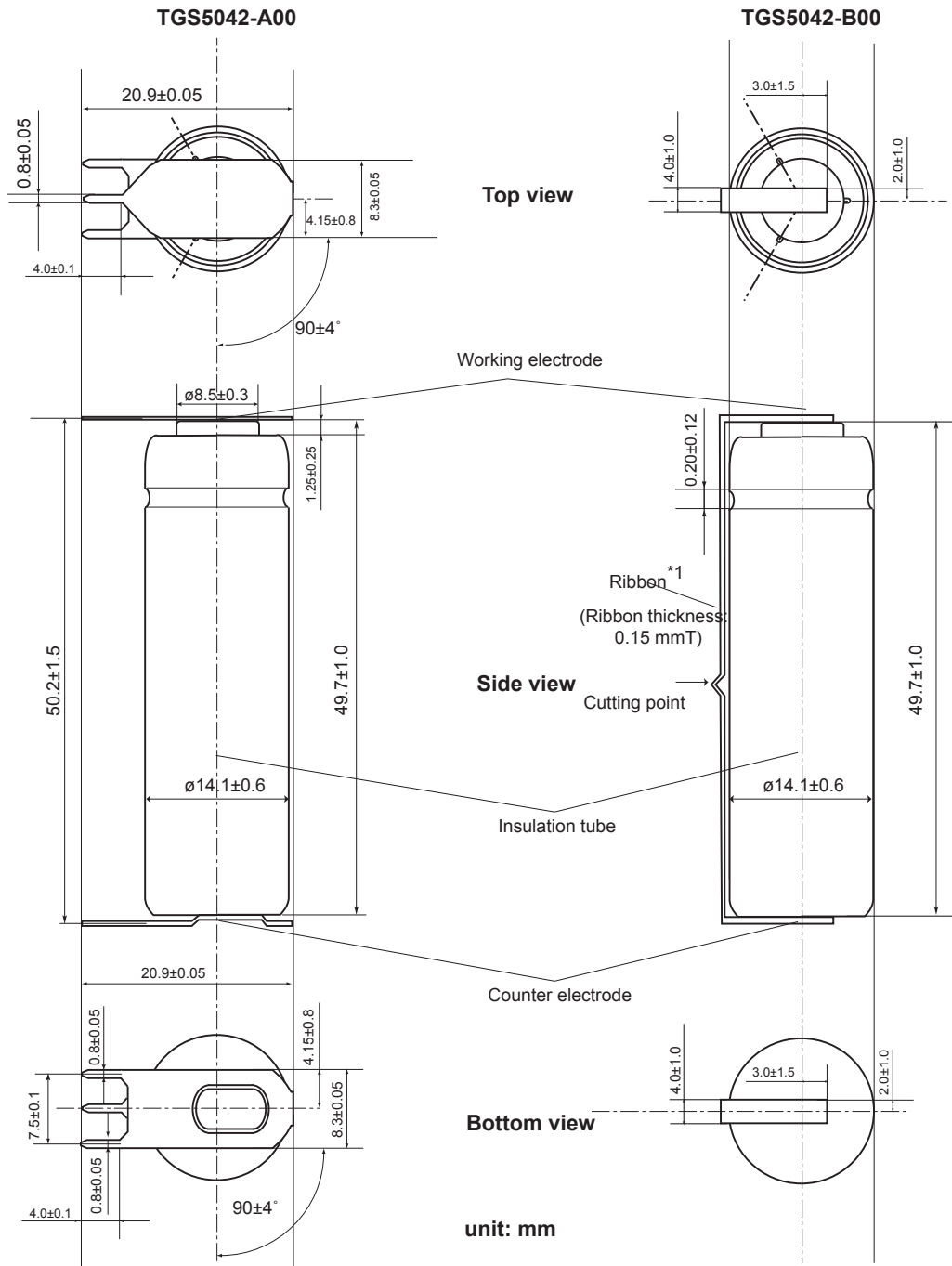
Figure 24 - TGS5042 Dimensions (lead configurations)
