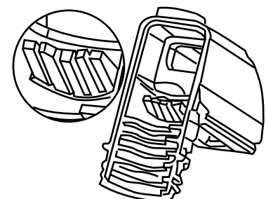
Strain Relief
