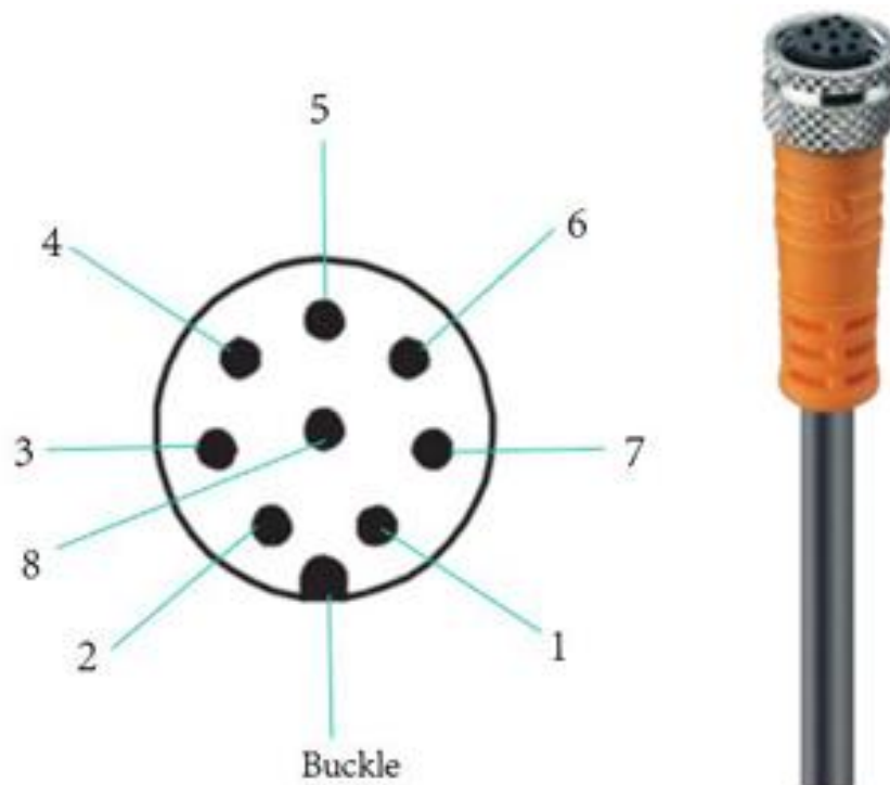
Figure 3.6 Lumberg RKMV 8-354 I/O pins
