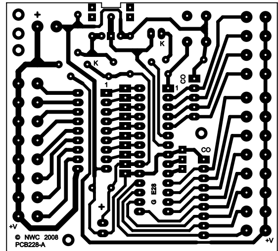
PCB artwork (viewed from copper side):
