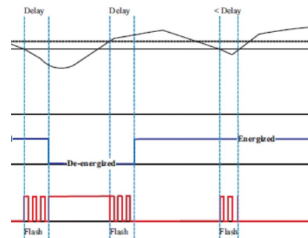
Under mode working timing diagram
