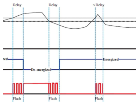
Over mode working timing diagram
