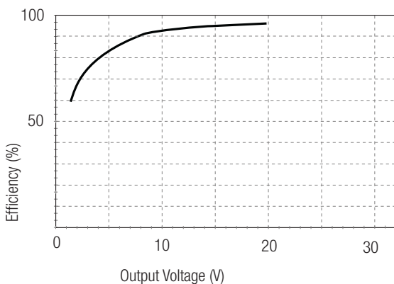
V_{in} = 24V, I_{out} = 300\sim 700mA
