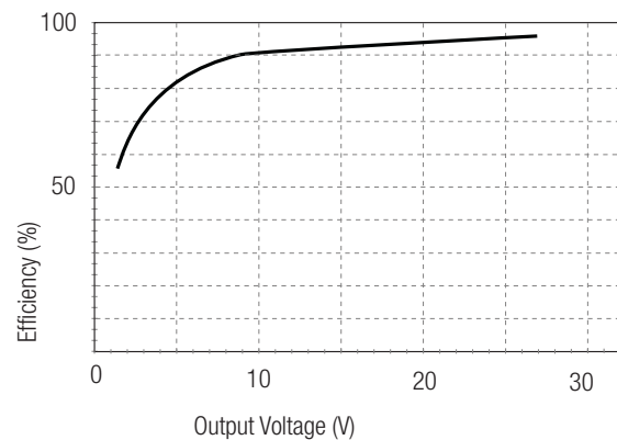
V_{in} = 32V, I_{out} = 300\sim 700mA
