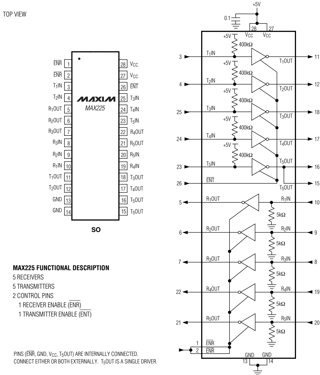
Figure 7. MAX225 Pin Configuration and Typical Operating Circuit
