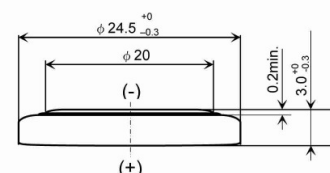
Dimension Drawing
