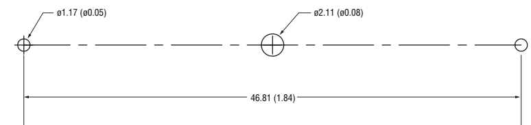
PCB LAYOUT
