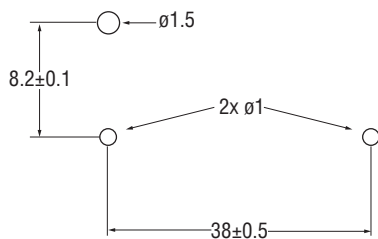
PCB/Mounting Layout
