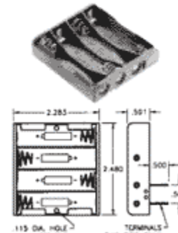
Holds Four (4) "AA" Cells in Series
