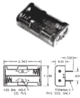
Holds Two (2) "AA" Cells in Series
