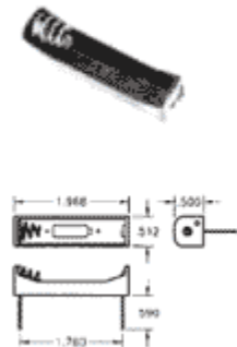
Holds One (1) "AAA" Cells
