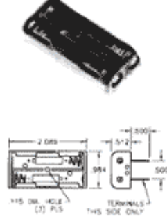
Holds Two (2) "AAA" Cells in Series
