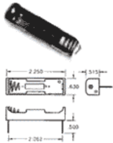
Holds One (1) "AA" Cell
