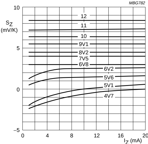
BZX55-C4V7 to C12. T_j = 25 to 150\text{ }^{\circ}\text{C} .
