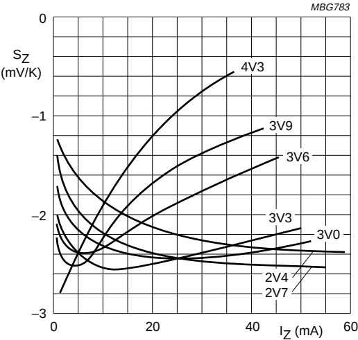
BZX55-C2V4 to C4V3. T_j = 25 to 150\text{ }^{\circ}\text{C} .
