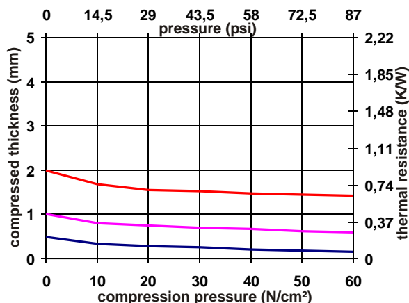
Compressibilities of Softtherm ® 86/500
