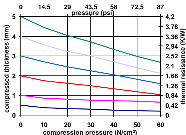
Compressibilities of Softtherm ® 86/300
