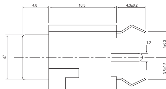
Schematic
