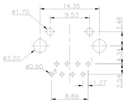
PC Board Layout t=1.6 mm Component Side Show
