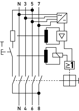
Wiring diagram
