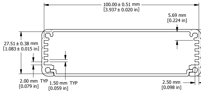
EXTRUSION
