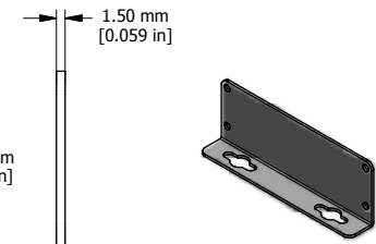
OPTIONAL FLANGE END PANELS 1455LF
