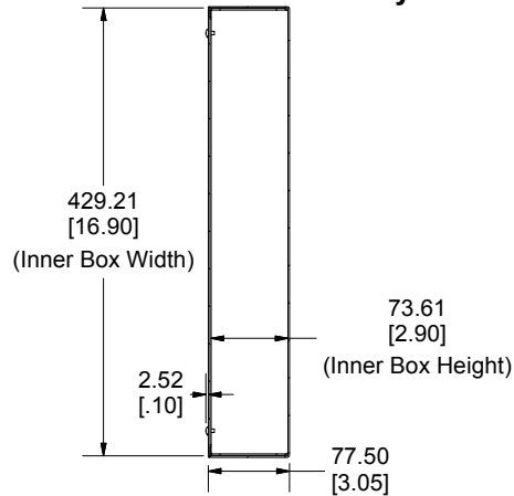
Bottom View of Chassis (Sold Separately)
