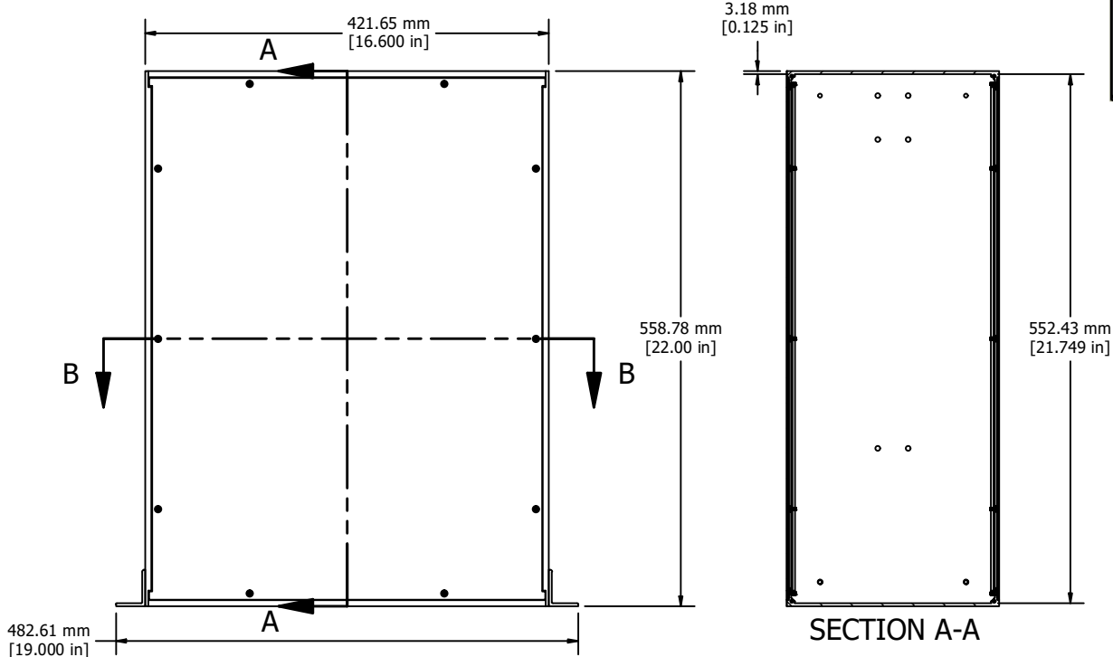
ASSEMBLY - TOP VIEW
