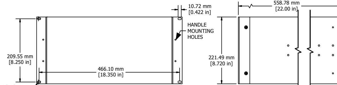
ASSEMBLY - FRONT VIEW
