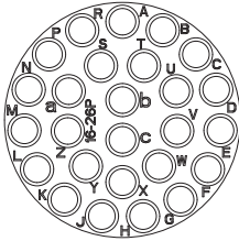
Connector on the HT4P main body side
