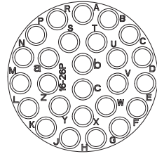
Connector on the HT4P main body side
