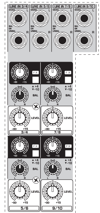
Fig. 2.2: Connectors and controls on the stereo channels
