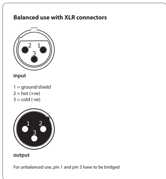
Fig. 4.1: XLR connections
