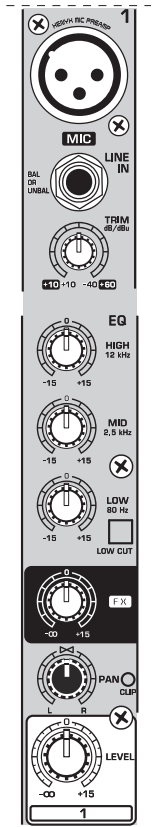
Fig. 2.1: Connectors and controls on the mono channels
