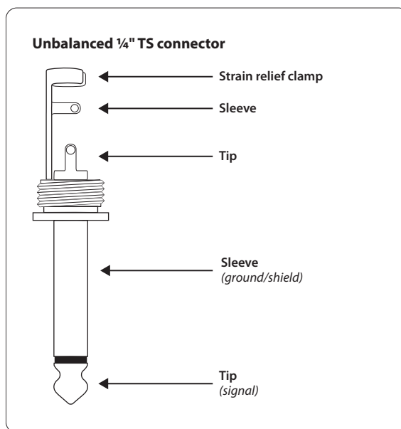
Fig. 4.3: ¼" stereo plug
