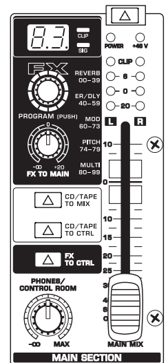
Fig. 2.4: Control elements of the main section
