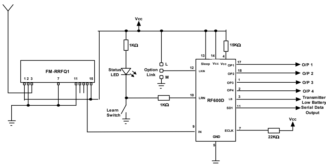
Receiver Circuit
