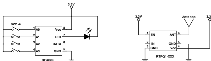
Transmitter Circuit
